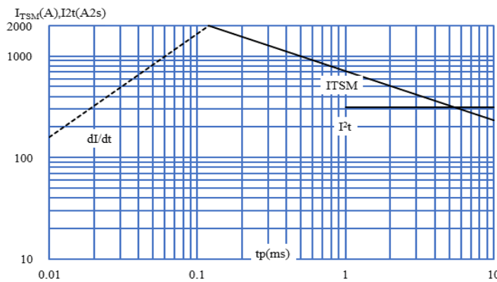
FIG.5: Non-repetitive surge peak on-state current for a sinusoidal pulse with width t_p < 20\text{ms} , and corresponding value of I^2t (I - II-III: dI/dt < 50\text{A}/\mu\text{s} ; IV: dI/dt < 10\text{A}/\mu\text{s} )
